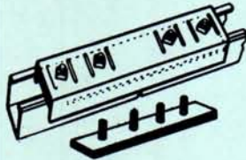
802 Joiner with Reinforcing Plate
