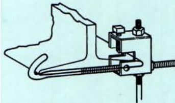
A-570 Beam Clamp with Safety Rods
