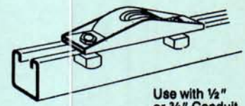
AB-315 Swing Connector
